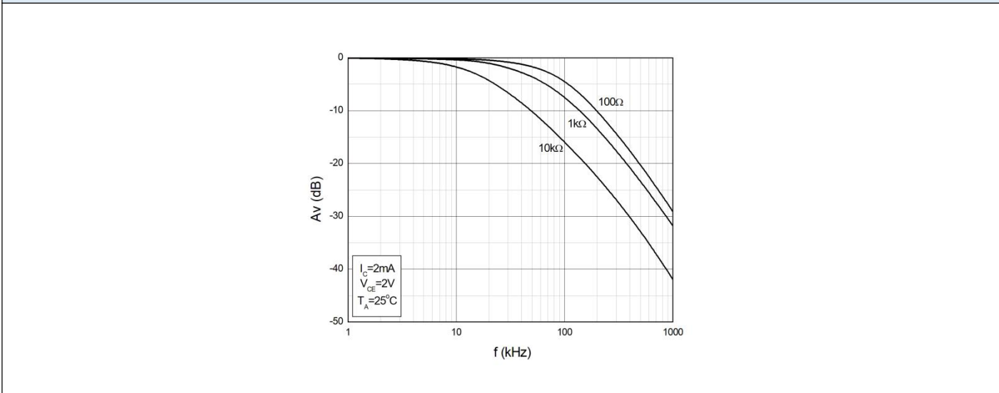
Fig.11 Frequency Response
